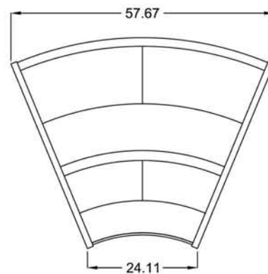
B - Server Side KD45EXT = 24.11"
