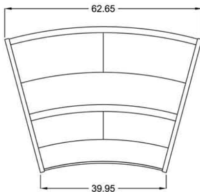
B - Server Side KD30EXT = 39.95"
